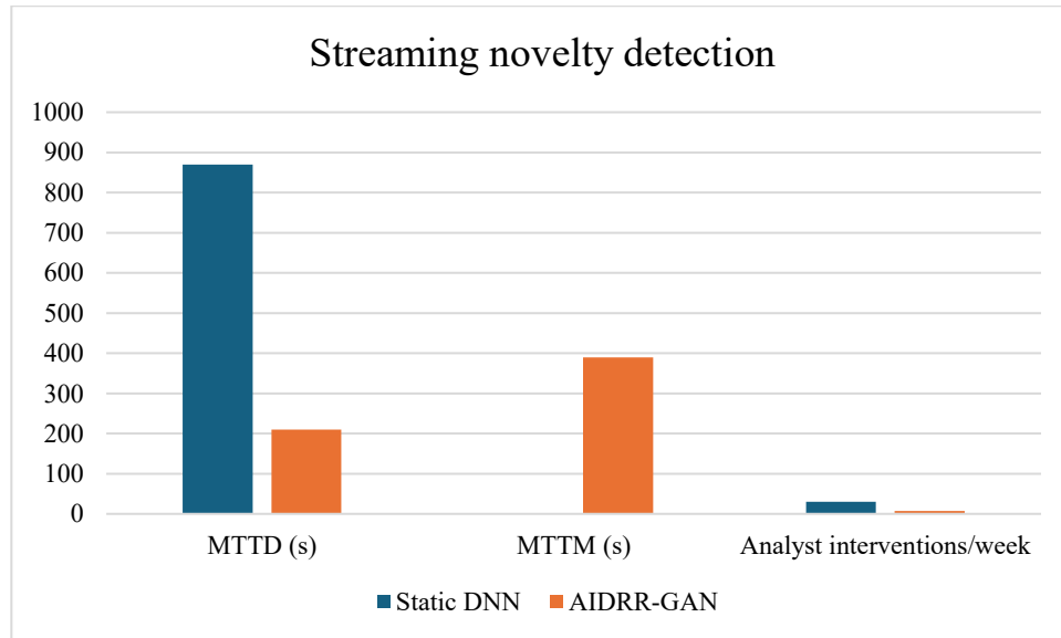
Fig.7.2: Streaming novelty detection
