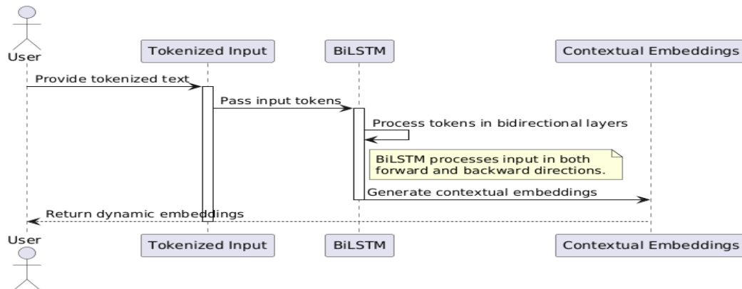
Figure 3. A UML sequence diagram illustrating ELMo's architecture
