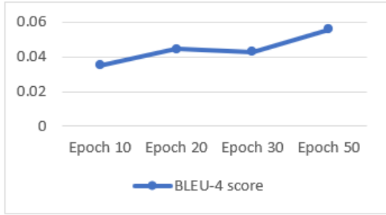
Figure 3: BLEU-4 score
