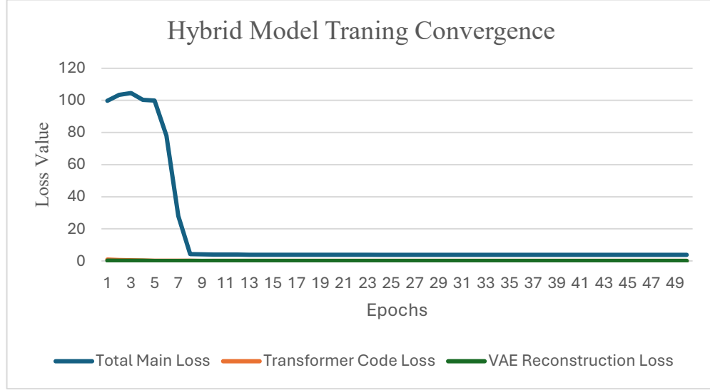
Figure 2: Training Losses
