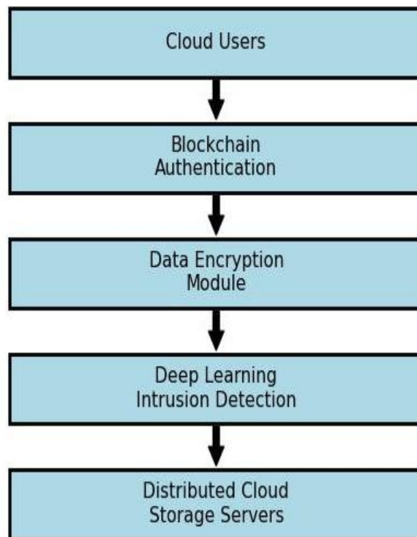
Figure 1. Proposed Secure Cloud Computing Framework Using Blockchain-Assisted Deep Learning
