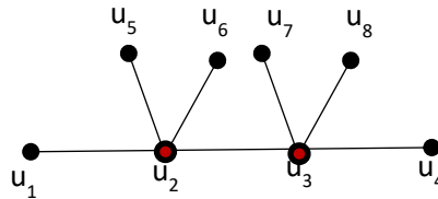
Figure 3. Connected Power Domination of Twig graph T_n .
