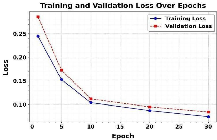
Figure 15: Training and Validation Loss across Epochs
