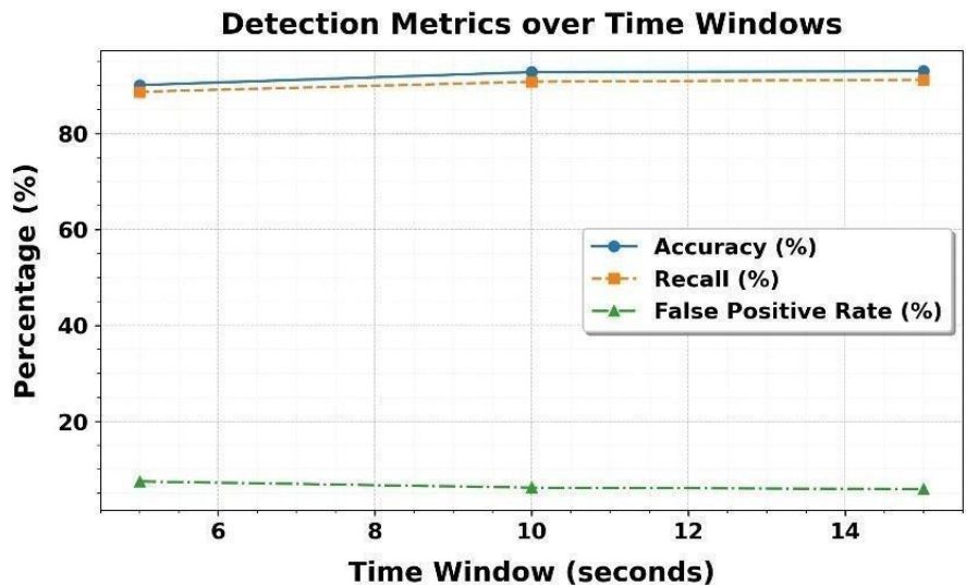
Figure 14: Detection Metrics Variation across Time Windows
