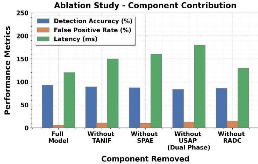
Figure 11: Component Impact on Intrusion Detection Performance
