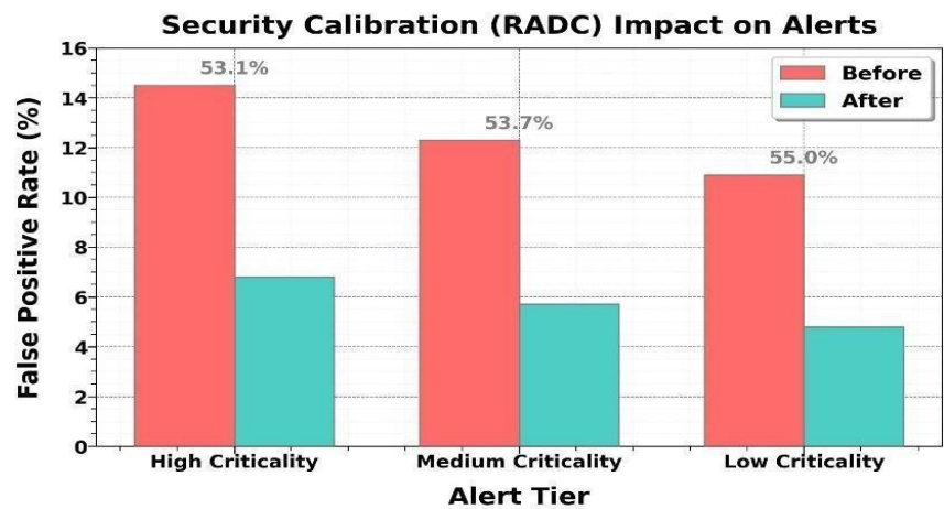
Figure 10: RADC Calibration Reduces False Positive Rates
