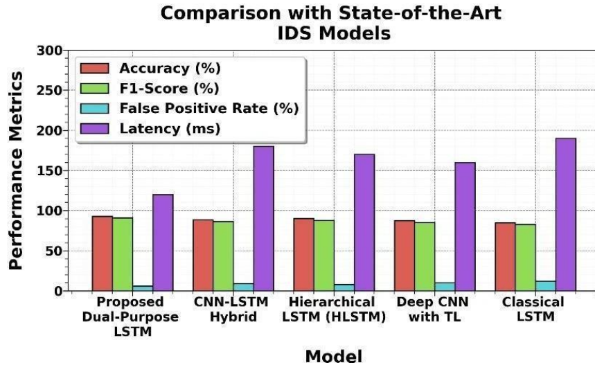
Figure 12: Performance Comparison of Advanced IDS Models
