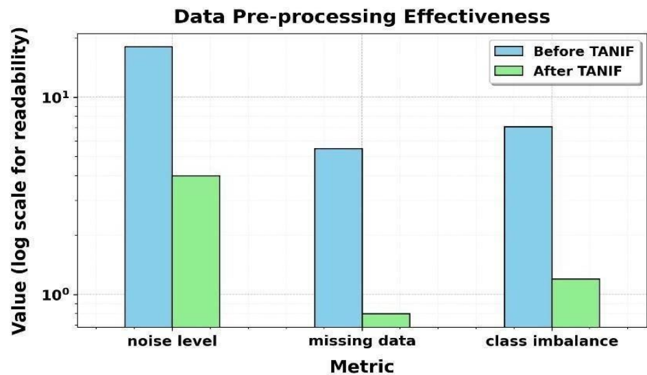
Figure 6: Enhanced Dataset Quality Using TANIF Preprocessing
