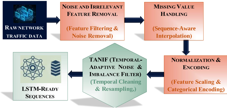
Figure 2: Temporal LSTM Data Pre-Processing Workflow
