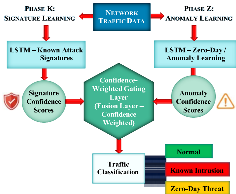
Figure 4: Dual-Phase LSTM Intrusion Detection Framework
