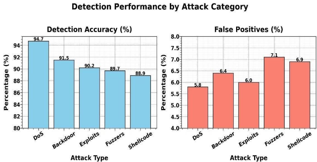
Figure 13: Detection Accuracy across Different Attack Types
