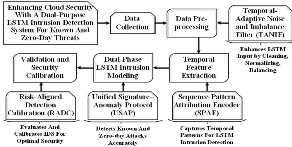
Figure 1: Block Diagram of the Proposed Work
