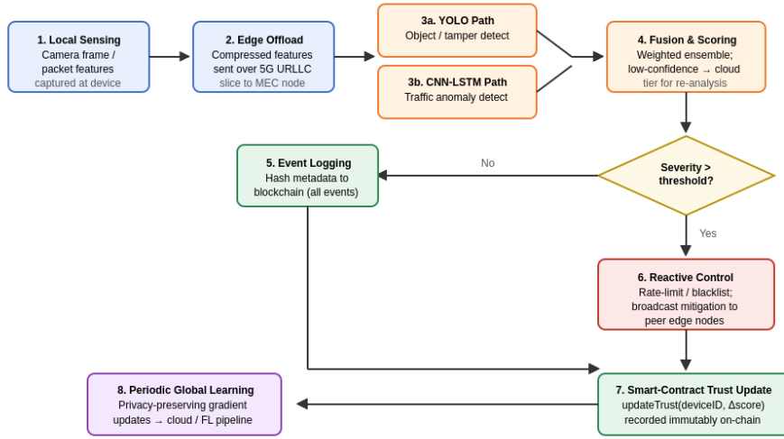
Figure 2. End-to-End Threat Detection and Trust-Update Workflow
