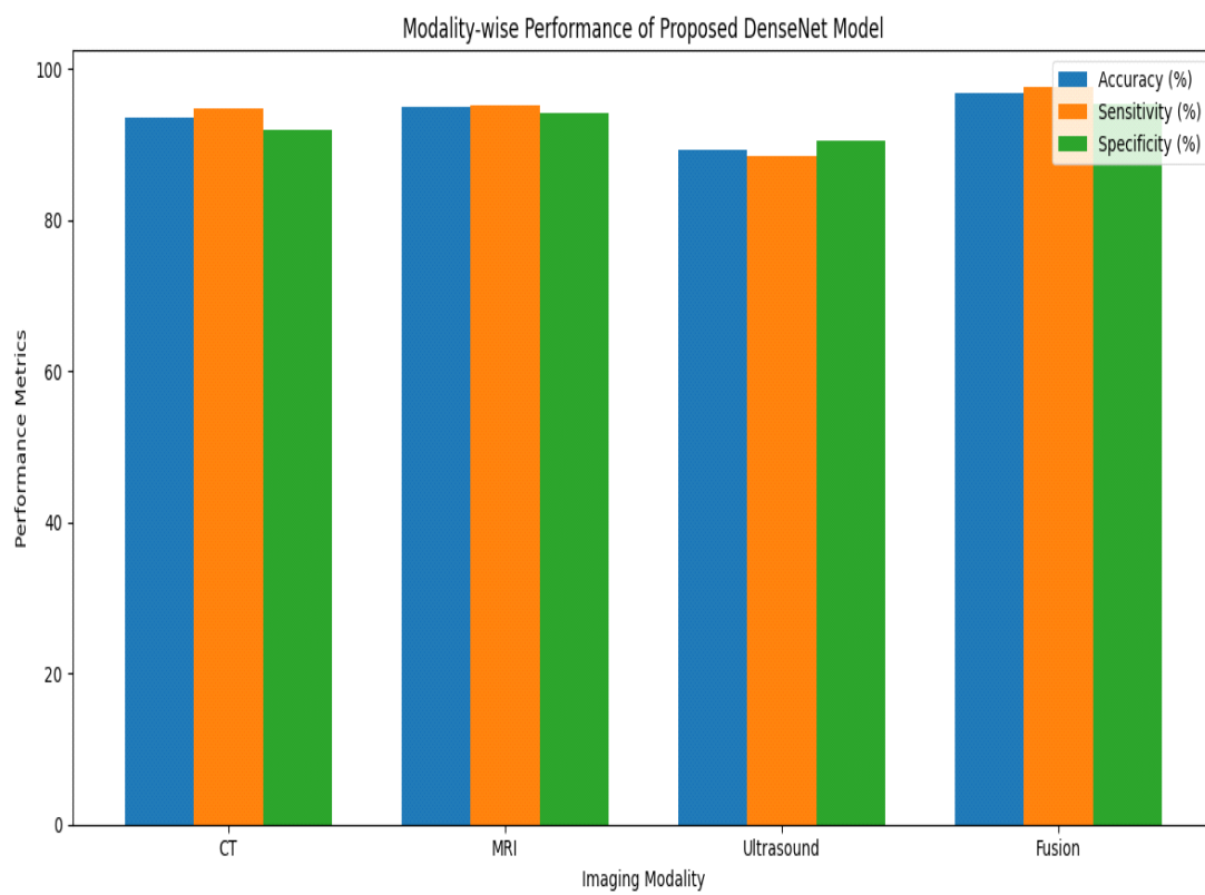
Fig 2. Modality-wise Performance of Proposed DenseNet
