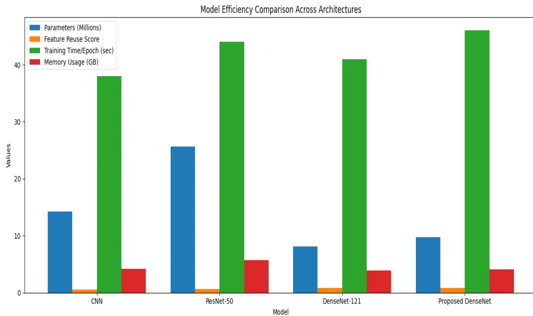
Fig 3. Feature Extraction Efficiency Across Models
