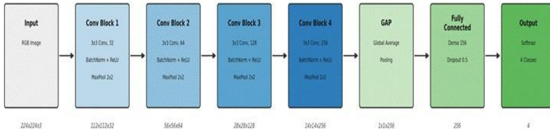
Figure 1. Schematic of the proposed deep convolutional neural network (DCNN) framework for crack detection and classification.
