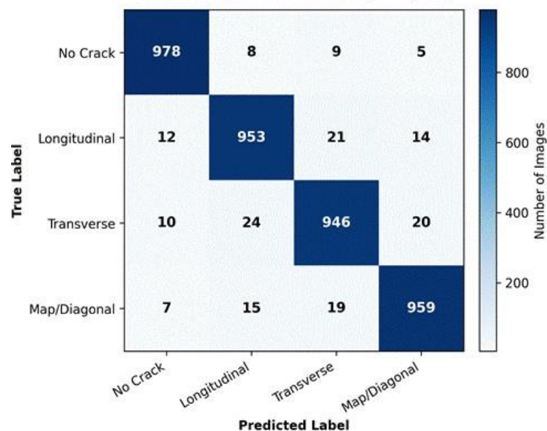
Figure 3. Confusion matrix of the proposed DCNN model on the independent test set (n = 4,000).
