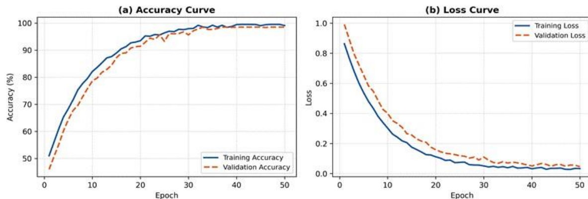
Figure 2. Training and validation accuracy and loss curves of the proposed DCNN model over 50 training epochs.
