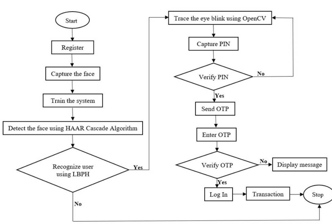
Fig: 3.1 Application Flow Diagram
