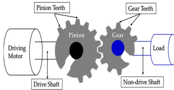
Figure1.5: The spur gearbox model.
