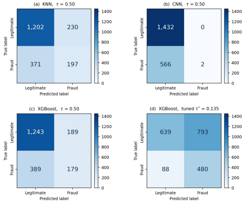
Figure 6. Confusion matrices on the held-out validation partition ( n = 2,000 ; 1,432 legitimate, 568 fraudulent). (a) KNN at \tau = 0.50 ; (b) CNN at \tau = 0.50 ; (c) XGBoost at the default threshold \tau = 0.50 ; (d) XGBoost at the tuned threshold \tau^* = 0.135 .
