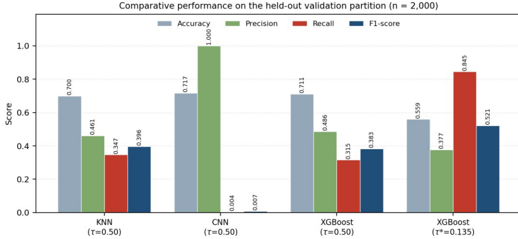
Figure 5. Comparative performance across the four configurations. The inverse relationship between accuracy and recall is visible directly.
