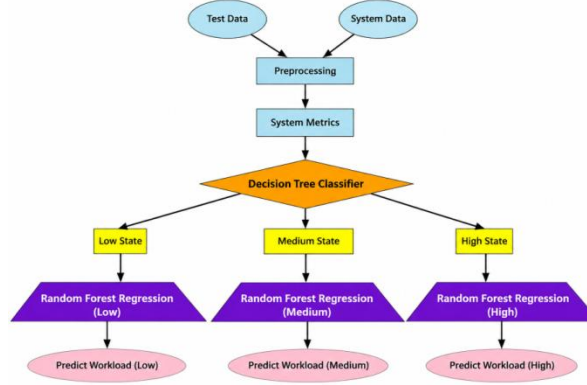
Figure 1. Architecture of the DTCRFR
