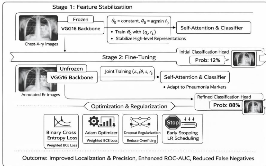
Figure 3. Two-stage training strategy and optimization framework for pneumonia detection.
