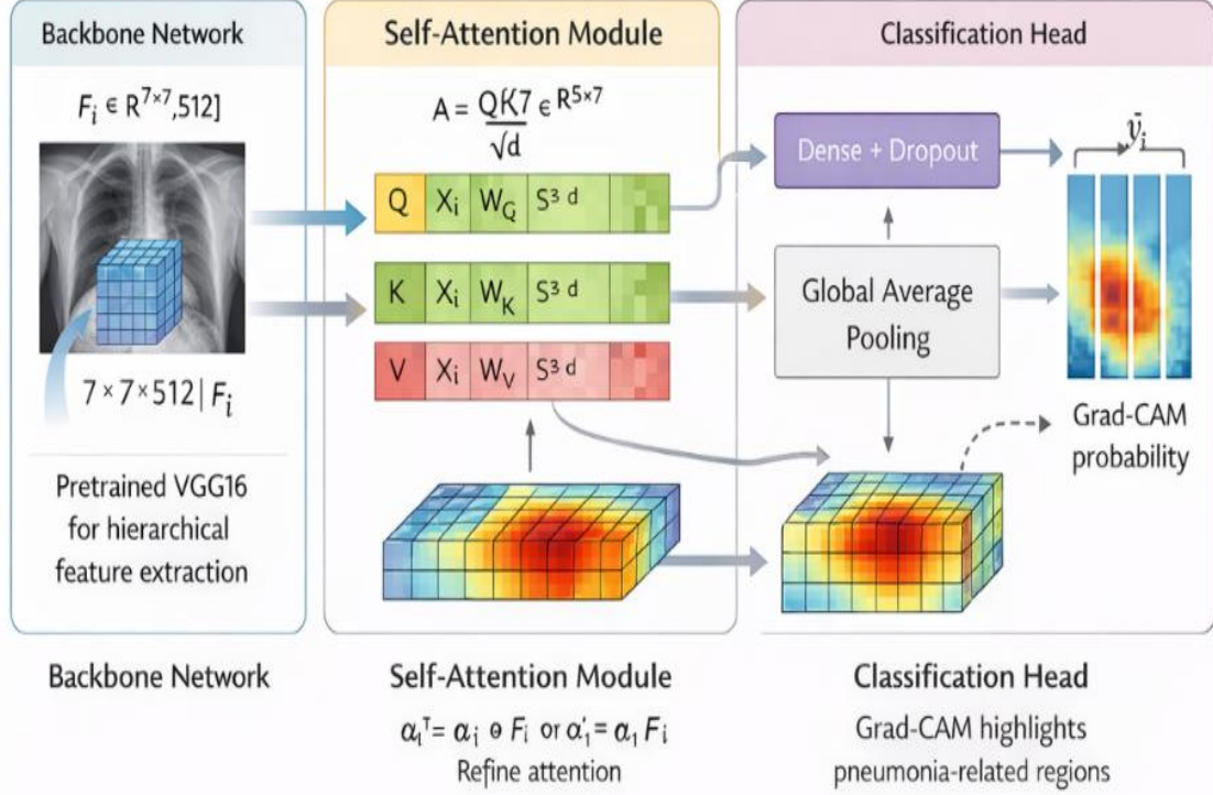
Fig.2. Attention-based pneumonia detection system
