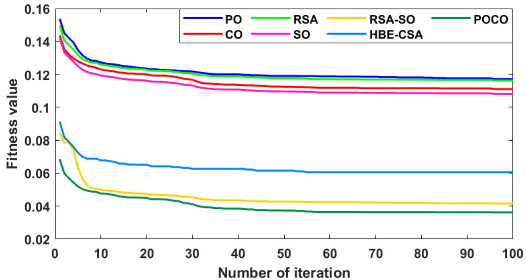
Fig. 4 Convergence curve of the various MHAs and PCO.
