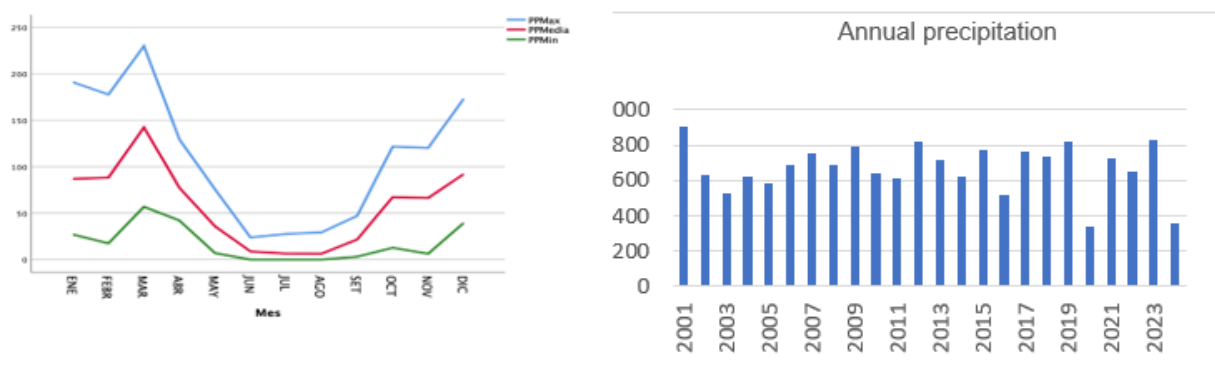
Fig. 1. Historical annual and monthly rainfall, maximum, average and minimum in mm. for the valley of Cajamarca - Peru.
