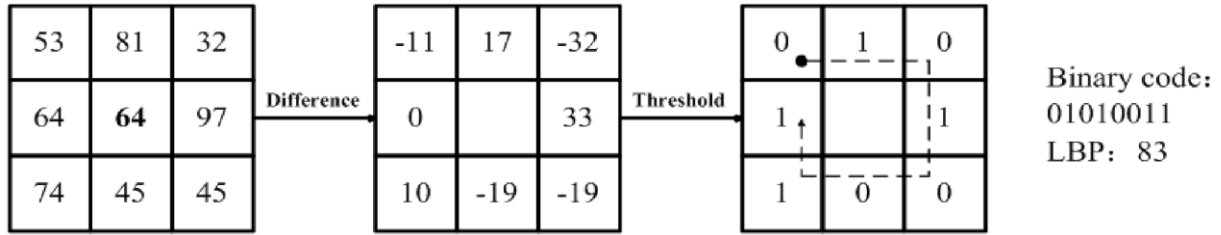
Figure 1: The generation of LBP value
