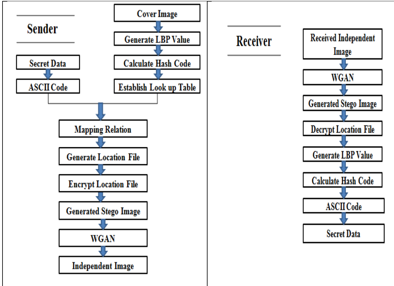
Figure 4: Proposed Method
