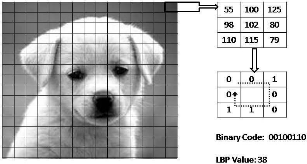
Figure 5: Calculation of a binary hash code
