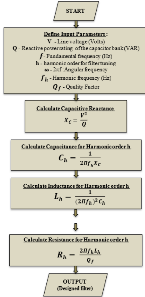
Fig. 4: Modelling of Single Tuned Filter
