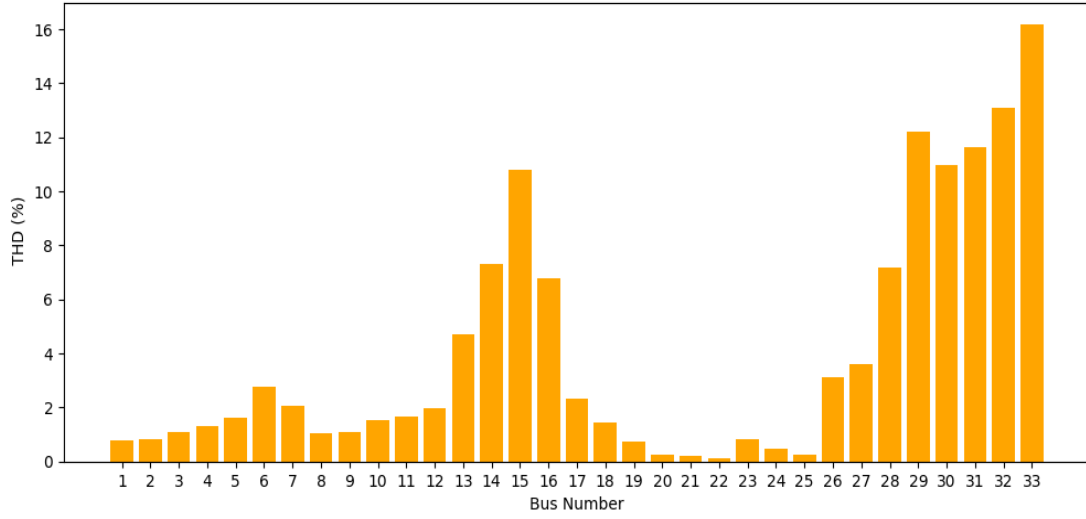
Fig. 5: Pre mitigation THD profile of the IEEE 33- bus ADN
