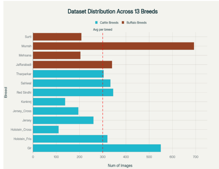
Fig 1: Dataset Distribution
