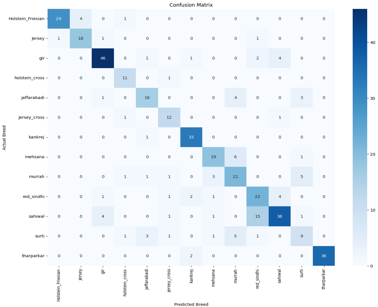
Fig 4: Confusion Matrix – InceptionResNetV2
