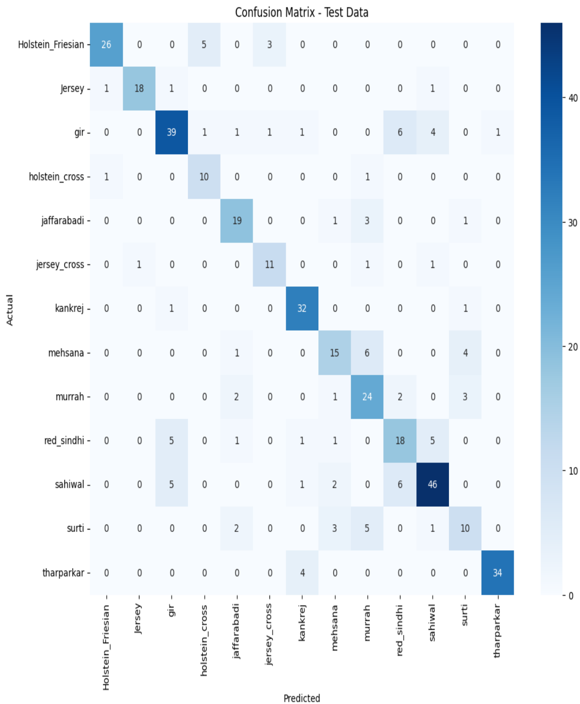
Fig 3: Confusion Matrix – ResNet50V2
