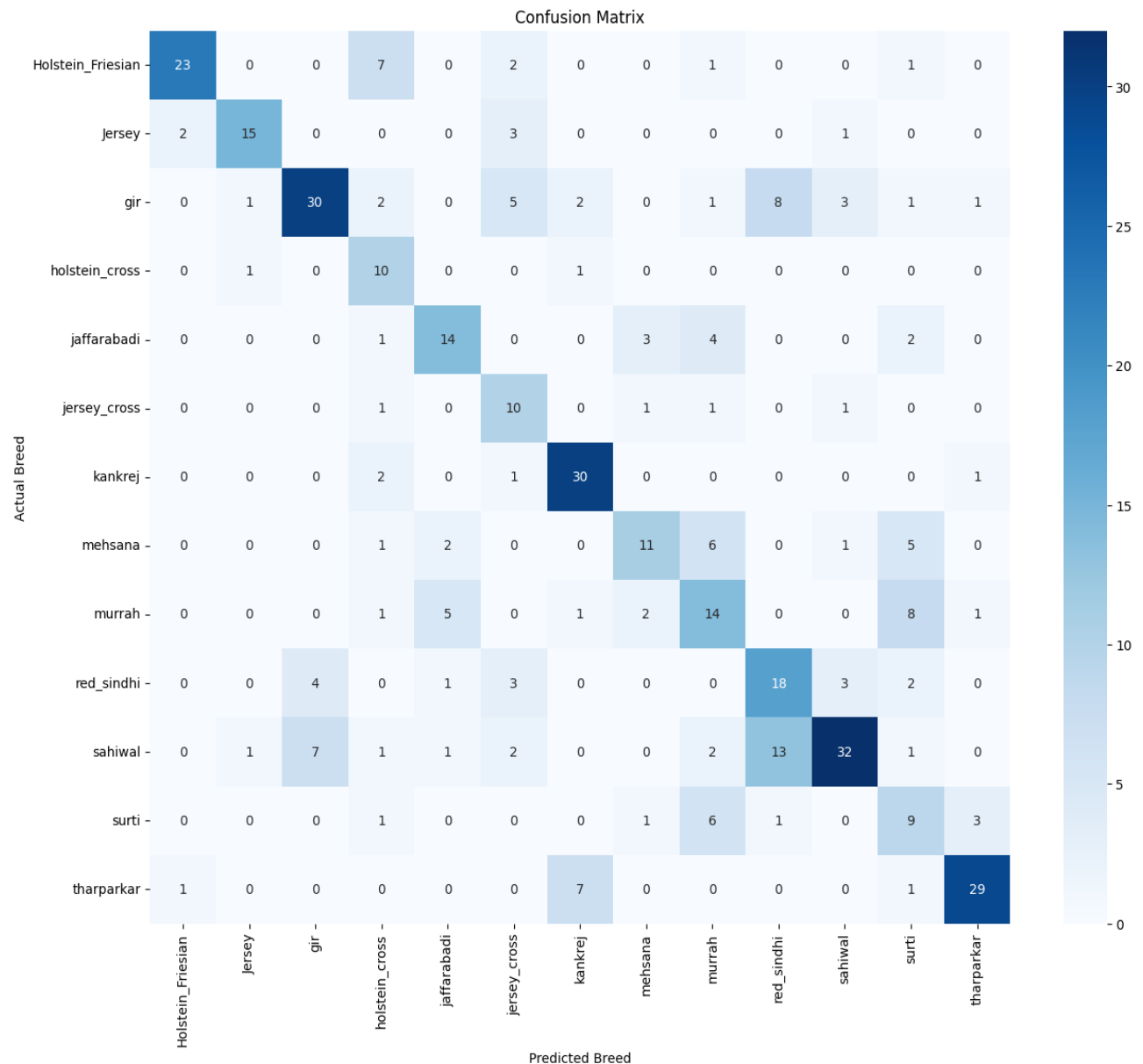
Fig 6: Confusion Matrix –ConvNeXtTiny
