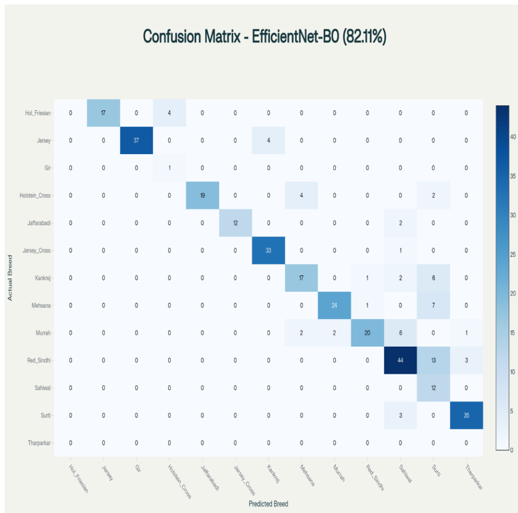
Fig 7: Confusion Matrix – EfficientNet-B0
