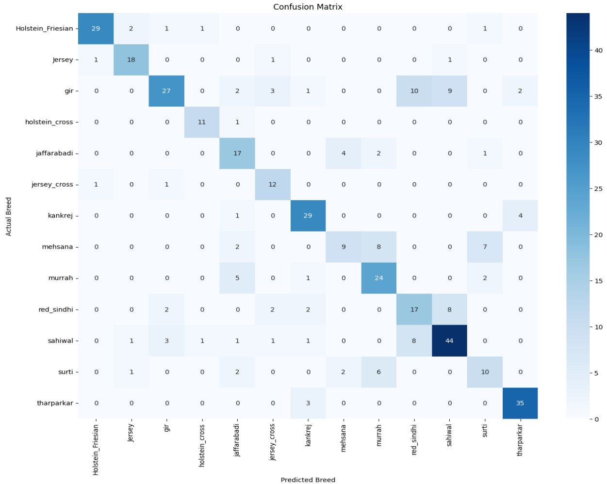
Fig 5: Confusion Matrix - MobileNetV2
