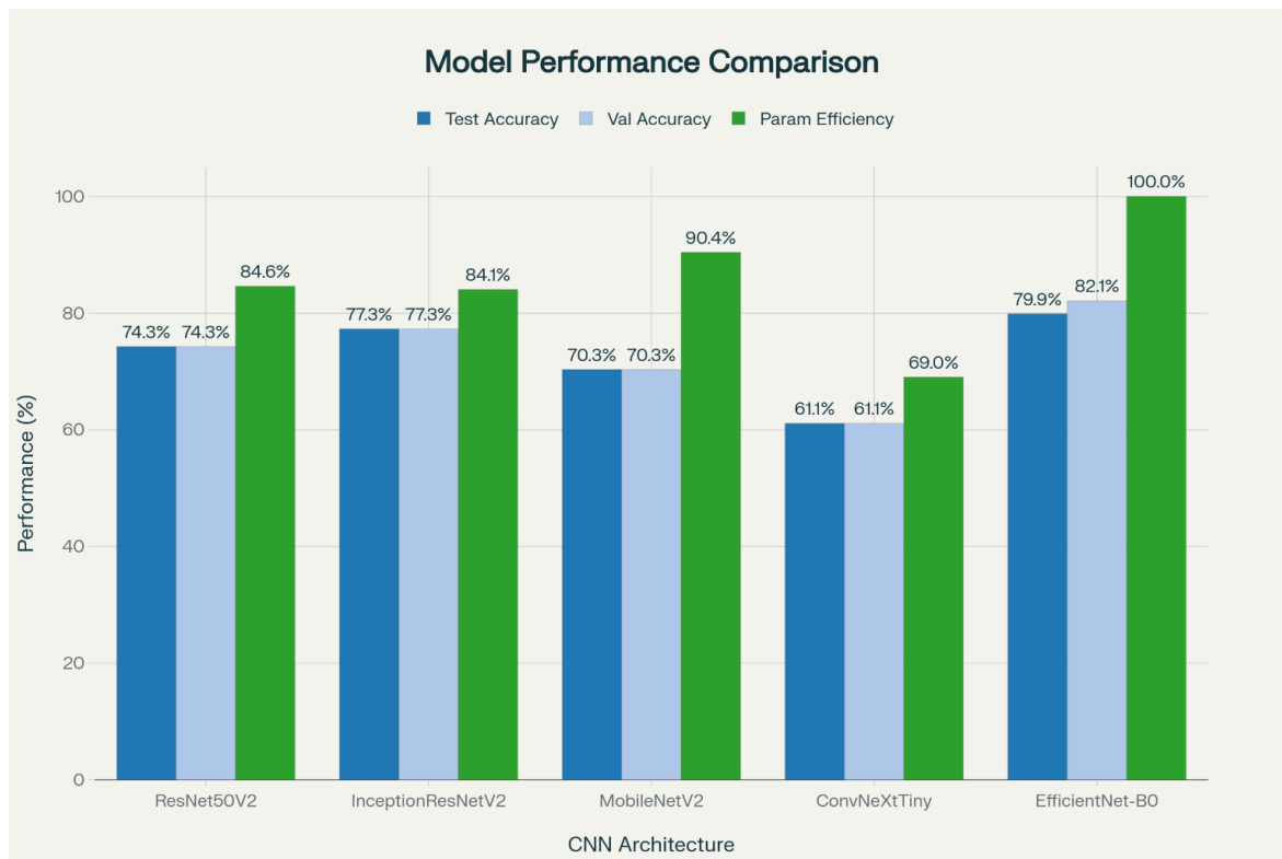
Fig 8: Model Performance Comparison
