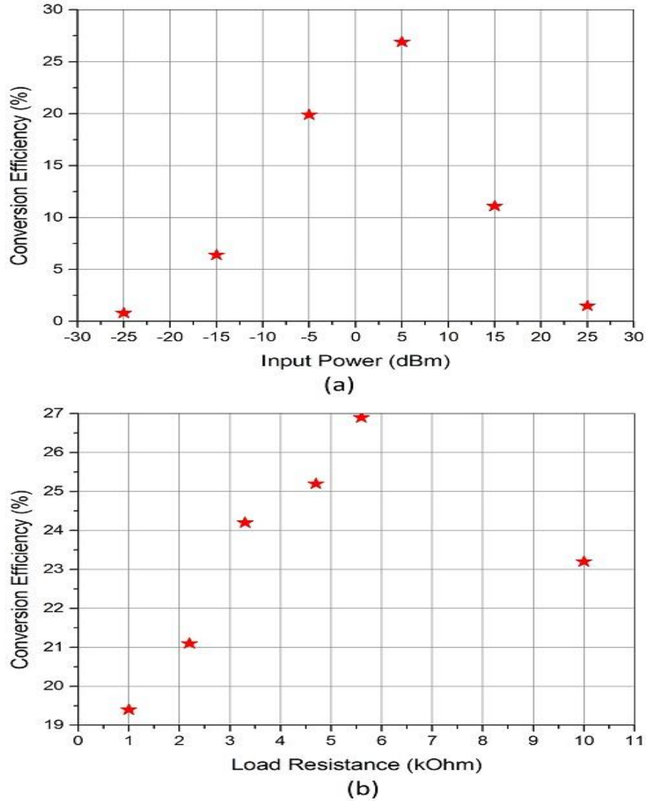
Figure. 9: Measurement results of rectenna (a) versus input power (b) versus load.
