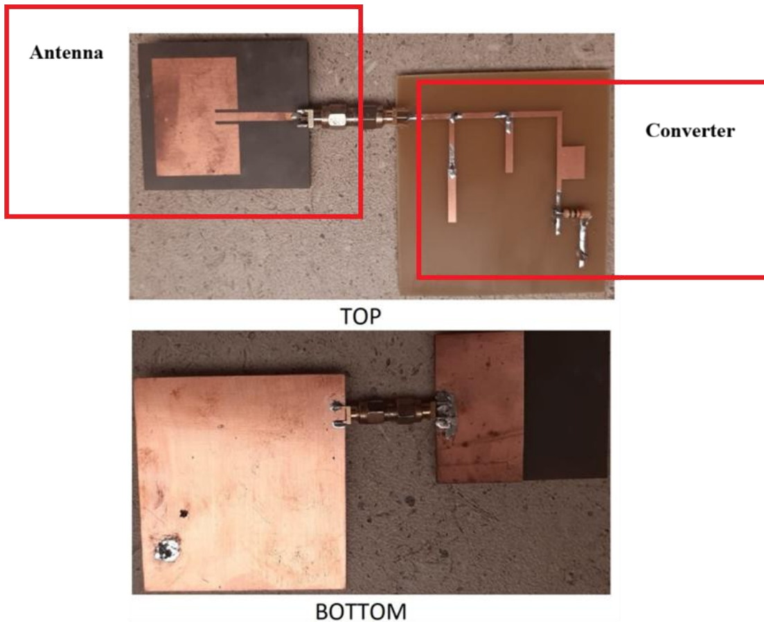
Figure.7: Fabricated proposed rectenna model.
