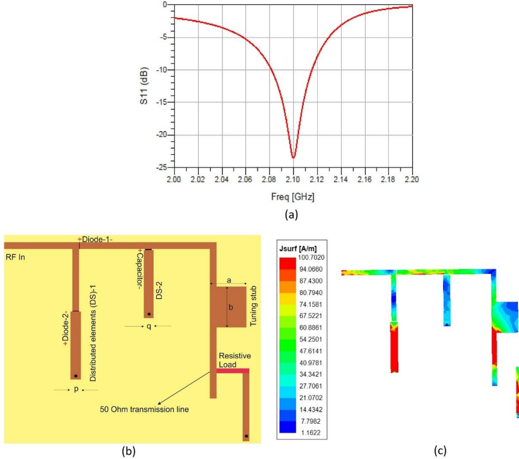
Figure. 2: Half-wave rectifier distributed element layout and performance parameters (a) S11 parameter (b) layout (c) Surface current density.
