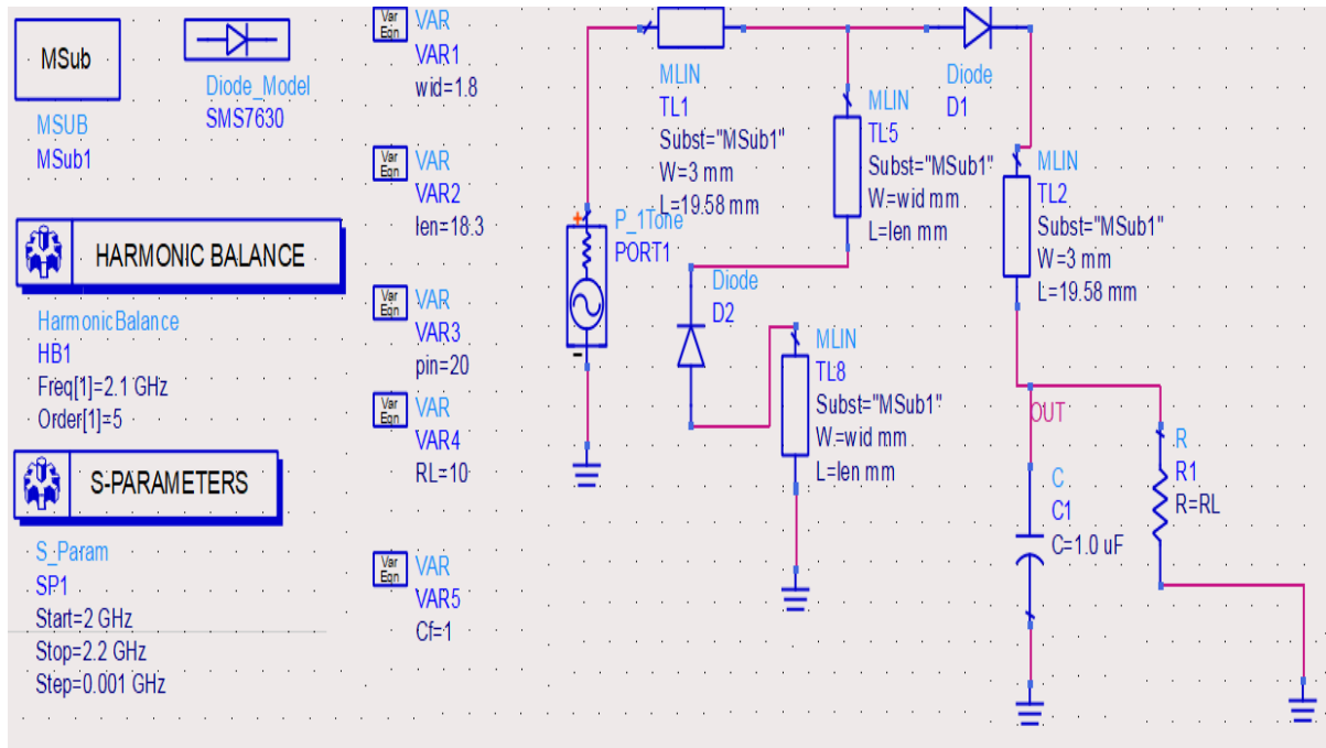
Figure. 1: Half-wave rectifier circuit diagram analysed using ADS.
