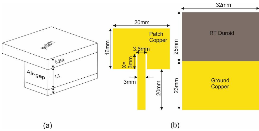
Figure. 4: Wideband high-gain antenna (a) Substrate (b) Antenna design.
