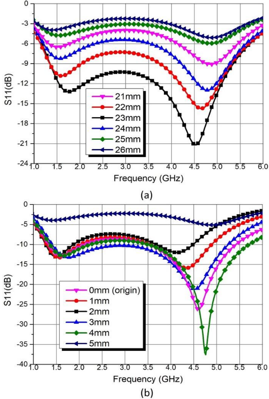
Figure. 5: Reflection coefficient of the wideband antenna (a) Versus ground size (b) Versus feeding position.
