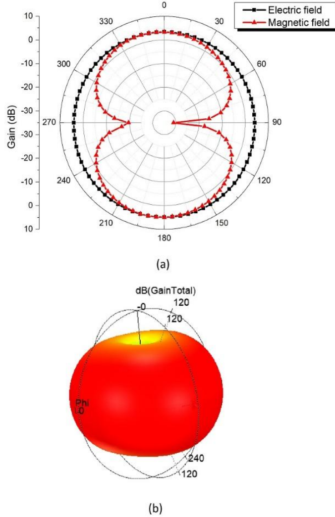
Figure. 6: Radiation patterns of the wideband antenna (a) Two dimensional electric and magnetic field pattern (b) three-dimensional radiation pattern.
