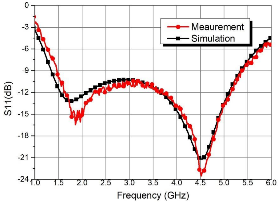
Figure. 8: Simulation and measurement S11 of the wideband antenna.
