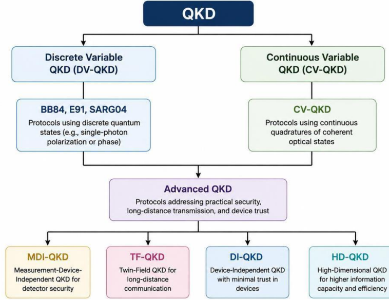
Figure 3. Classification of QKD protocols
