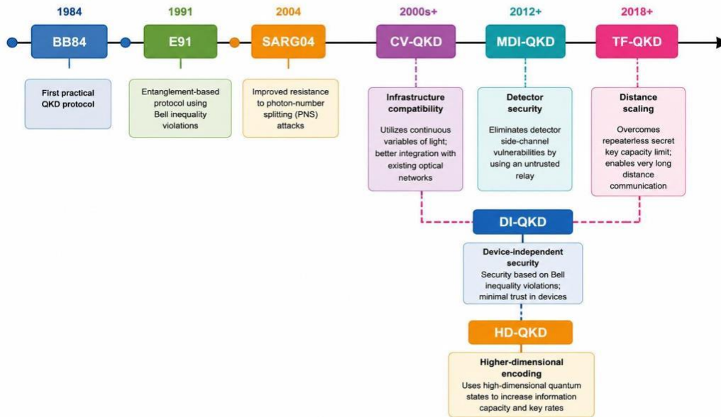
Figure 2. Evolution of QKD protocols and the problems addressed by each generation
