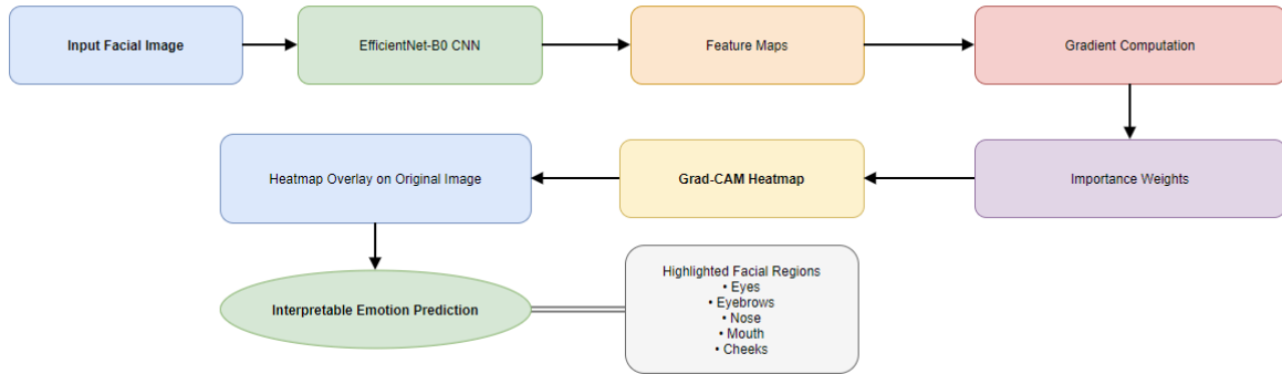
Figure 12: Grad-CAM Explainability Framework
