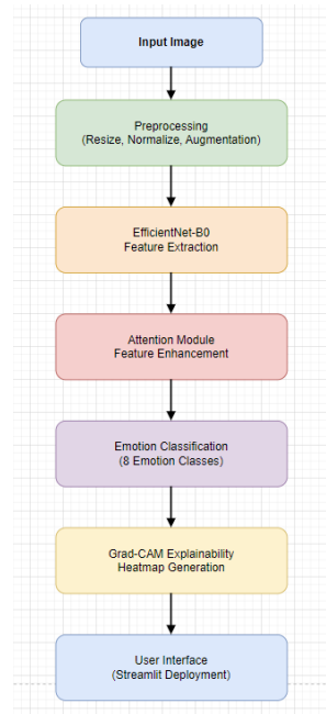
Figure 1: Proposed Facial Emotion Recognition Framework
