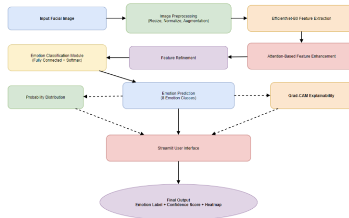
Figure 13: Overall Workflow of the Proposed FER System
