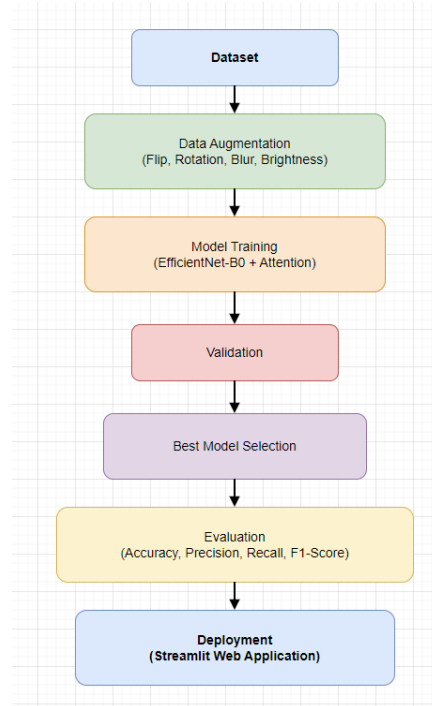
Figure 2: Emotion Recognition Pipeline
