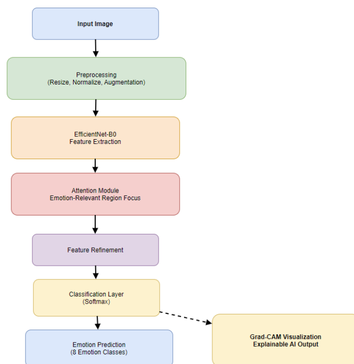
Figure 6: Proposed Facial Emotion Recognition Framework
