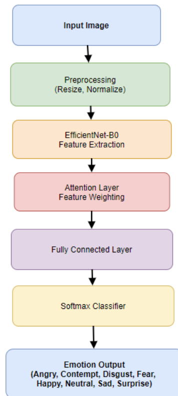
Figure 7: Generalized System Architecture
