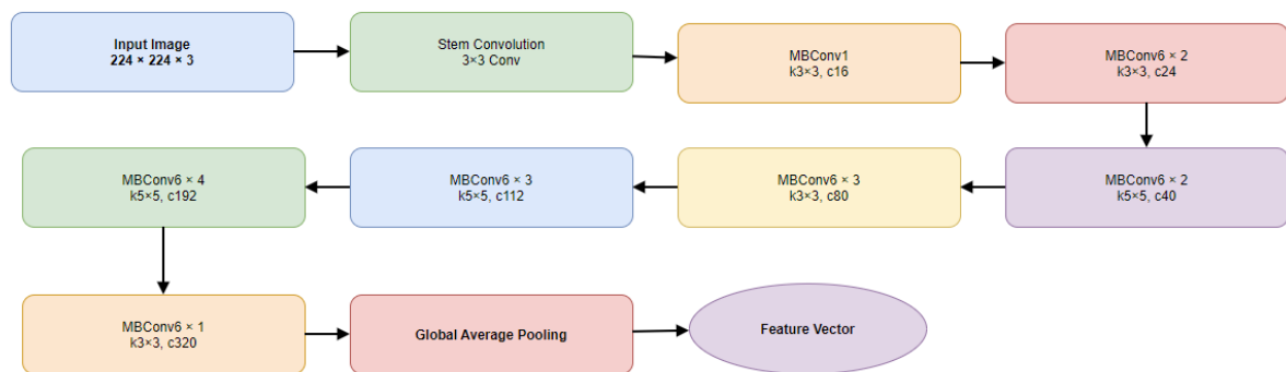
Figure 9: EfficientNet-B0 Architecture
