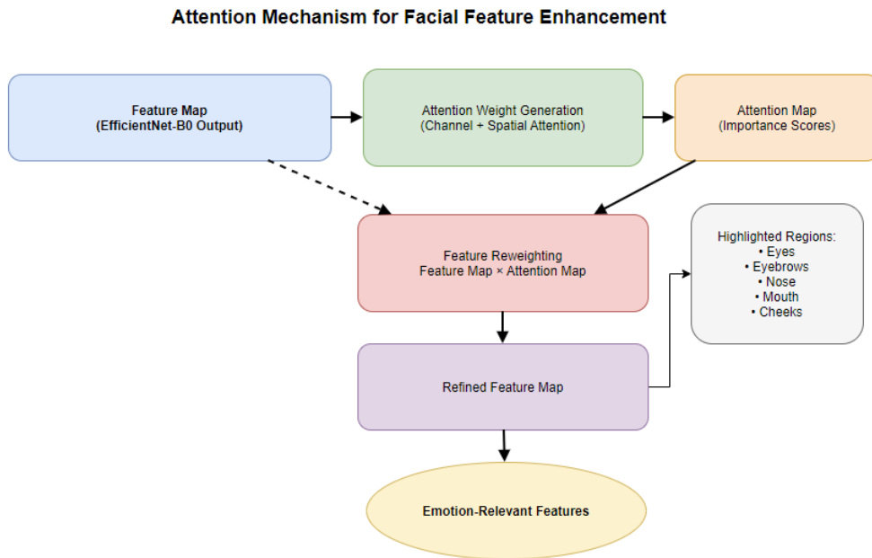
Figure 10: Attention Mechanism for Facial Feature Enhancement
