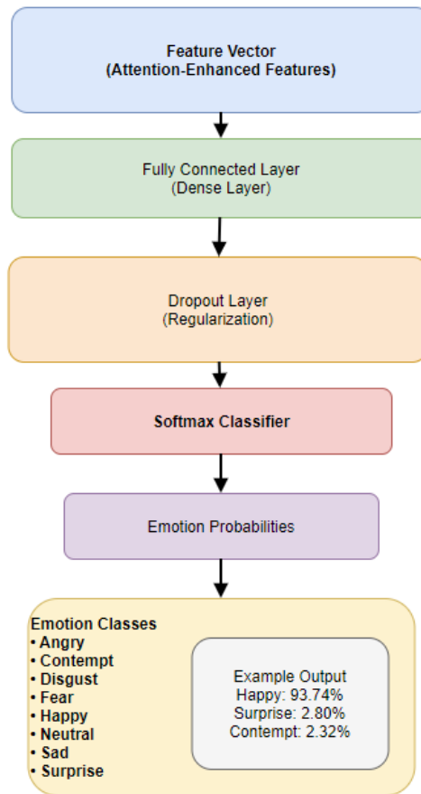
Figure 11: Emotion Classification Module
