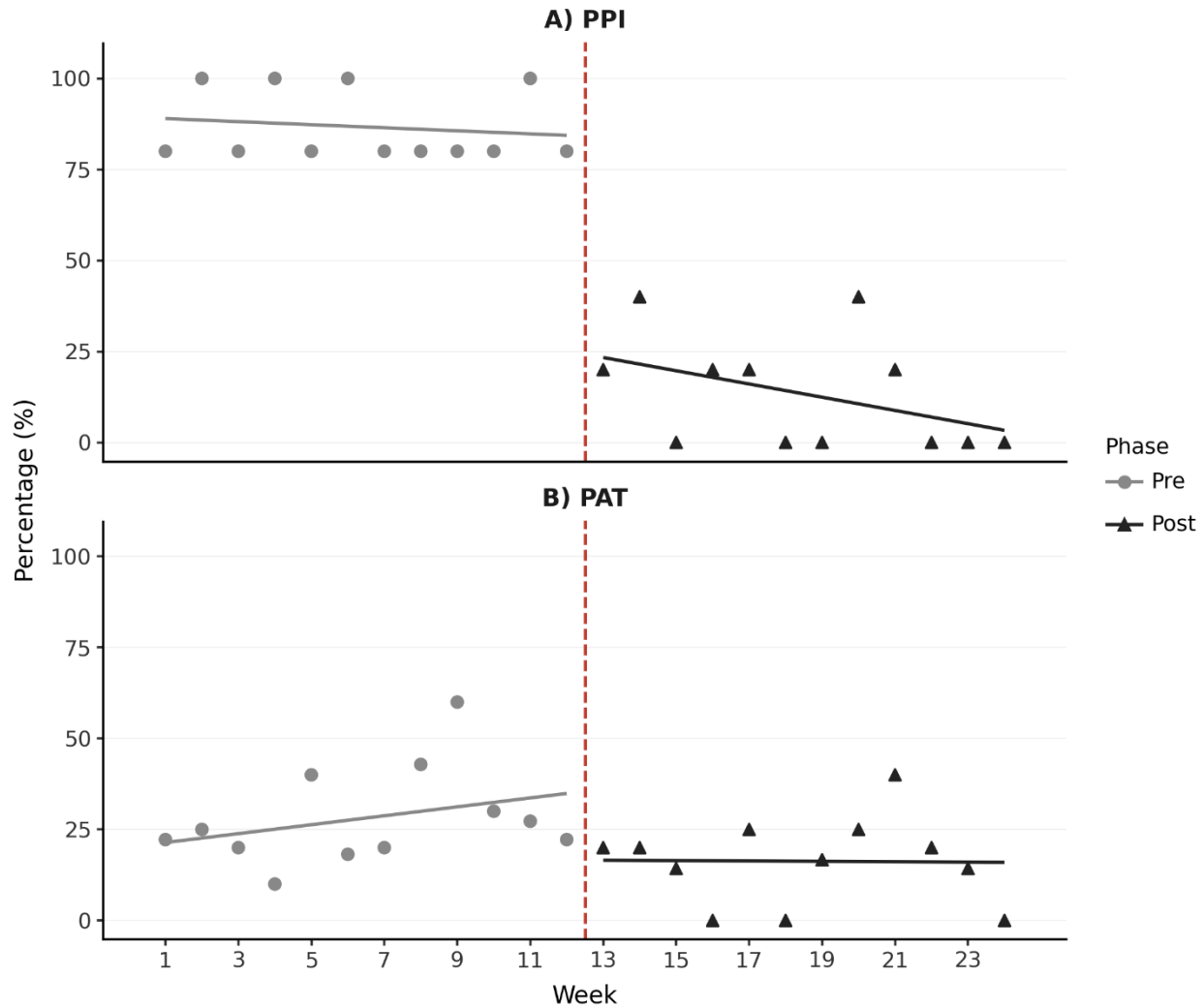
Title: Figure 3. Segmented interrupted time series for PPI (panel A) and PAT (panel B) across 24 weekly observations.
